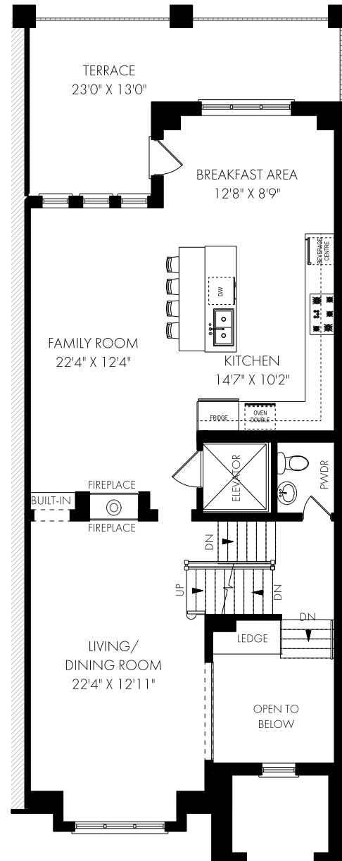
CEILING HEIGHT 10'0" MAIN FLOOR - 1109 SQUARE FEET
