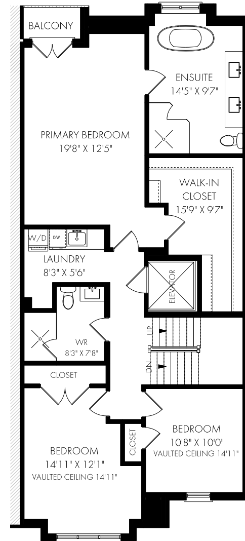
CEILING HEIGHT 9'0" SECOND FLOOR - 1242 SQUARE FEET
